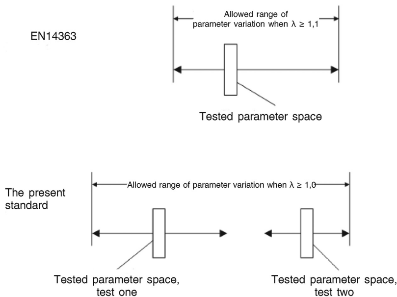
Parameter variation ranges for the acceptance after successful testing compared to the process in EN 14363:2005
